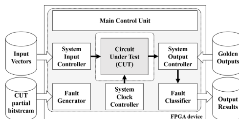
Fig. 3: Proposed fault injection infrastructure architecture
