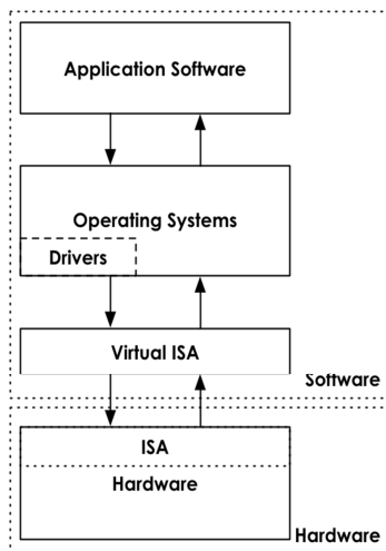
Figure 3: Virtualization of the Instruction Set Architecture
