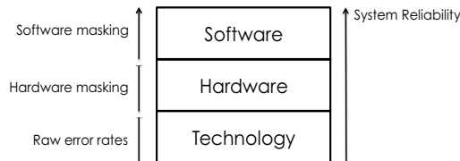
Figure 2: Masking effects in a computer system
